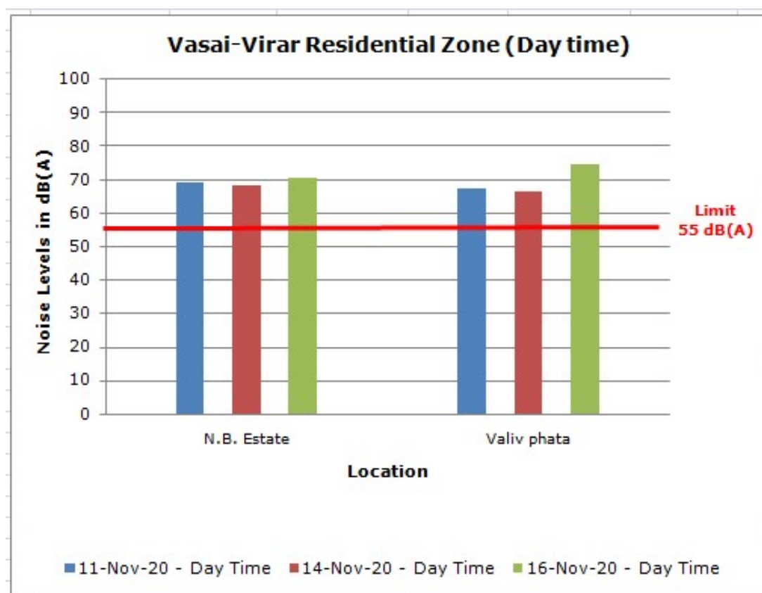
Chart 4.16: Noise Levels during Diwali Festival, 2020 in Vasai-Virar
