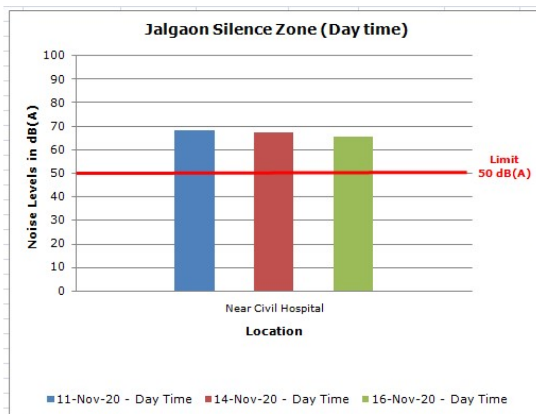
Chart 4.12: Noise Levels during Diwali Festival, 2020 in Jalgaon
