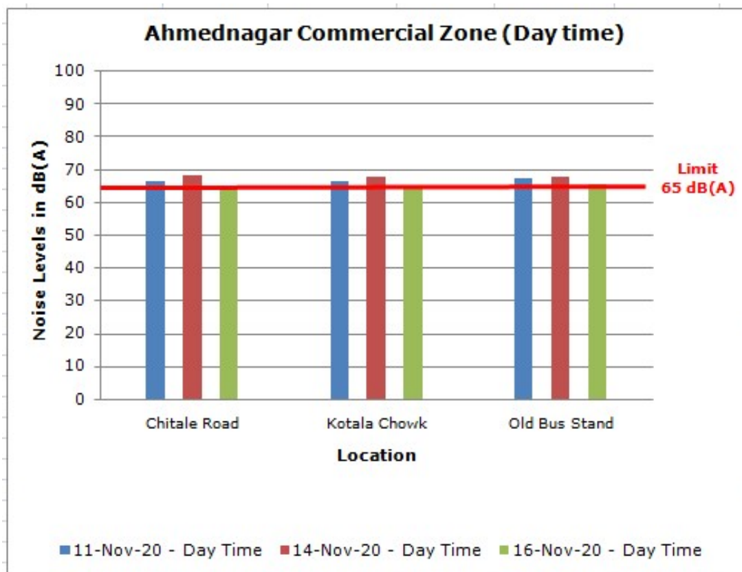
Chart 4.21: Noise Levels during Diwali Festival, 2020 in Ahmednagar
