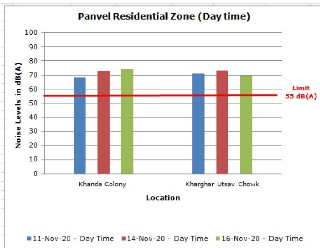
Chart 4.29: Noise Levels during Diwali Festival, 2020 in Panvel
