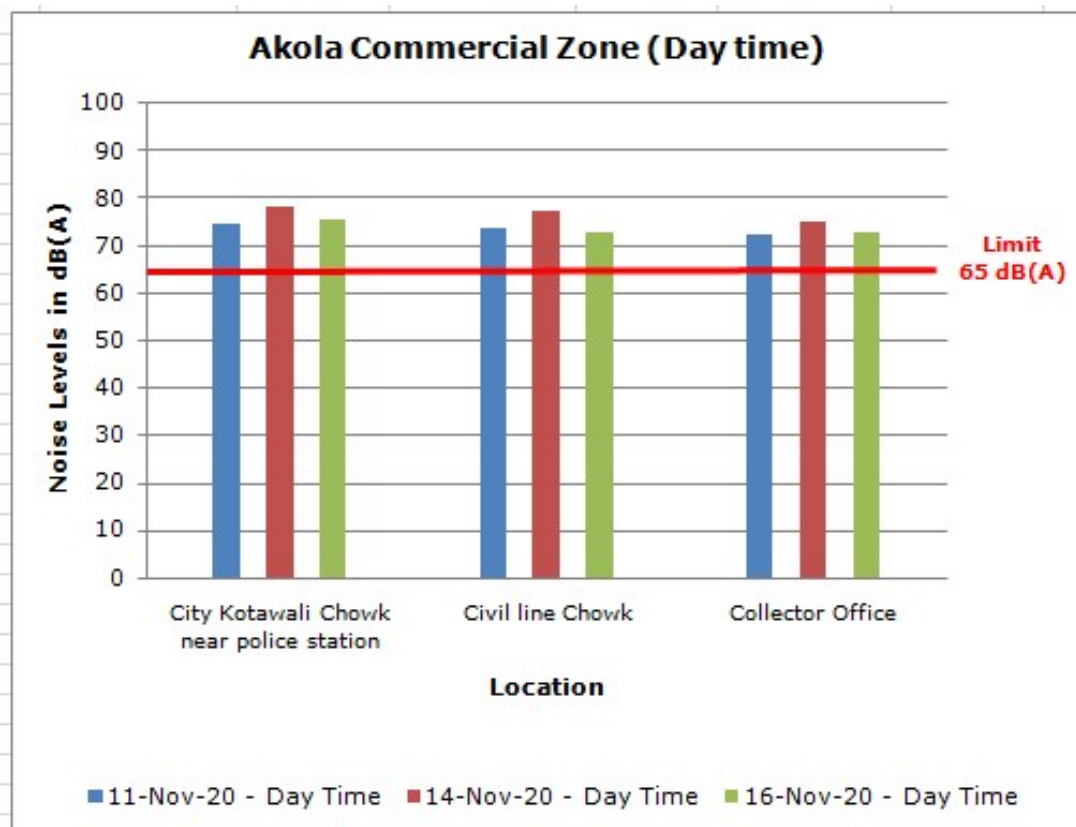
Chart 4.27: Noise Levels during Diwali Festival, 2020 Akola
