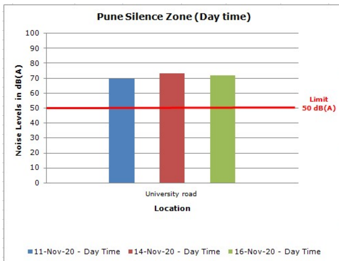
Chart 4.6: Noise Levels during Diwali Festival, 2020 in Pune
