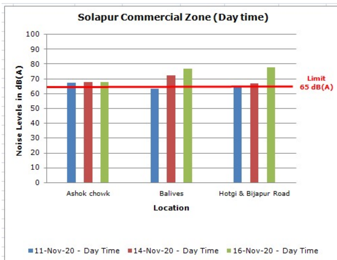
Chart 4.28: Noise Levels during Diwali Festival, 2020 in Solapur
