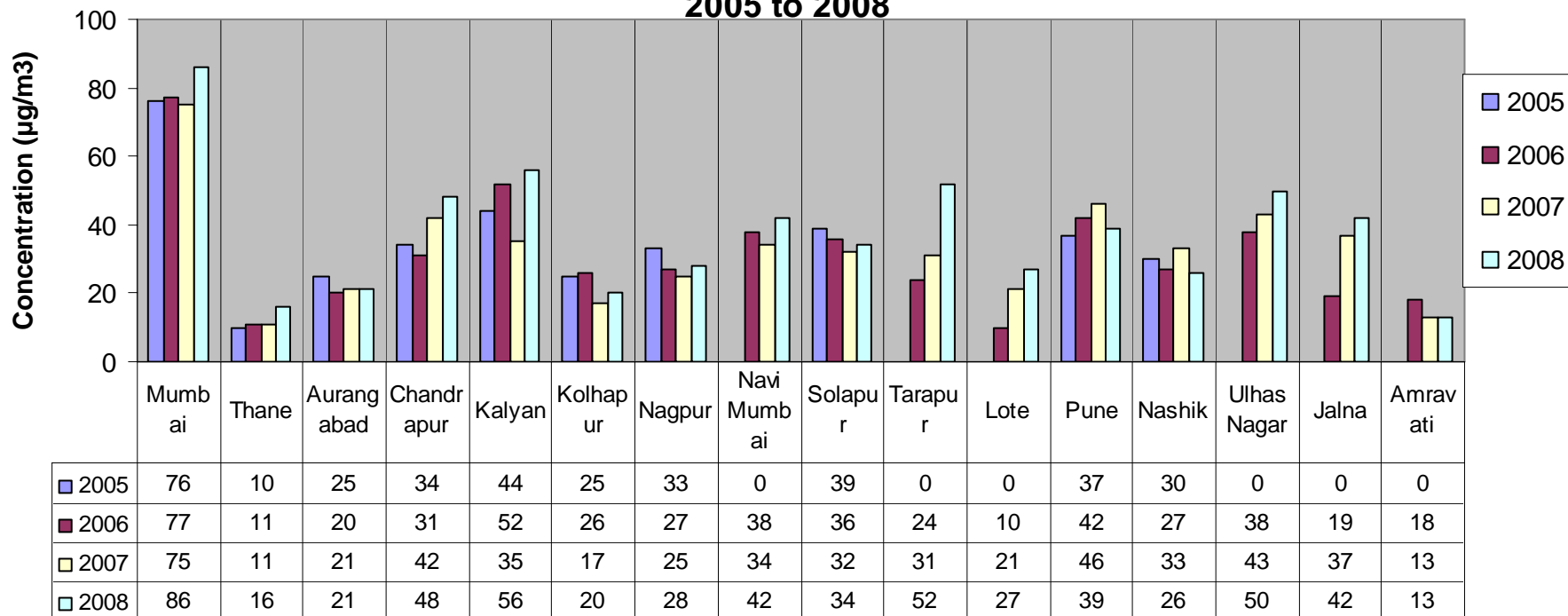
Trend in Annual Average concentration of Nox 2005 to 2008
