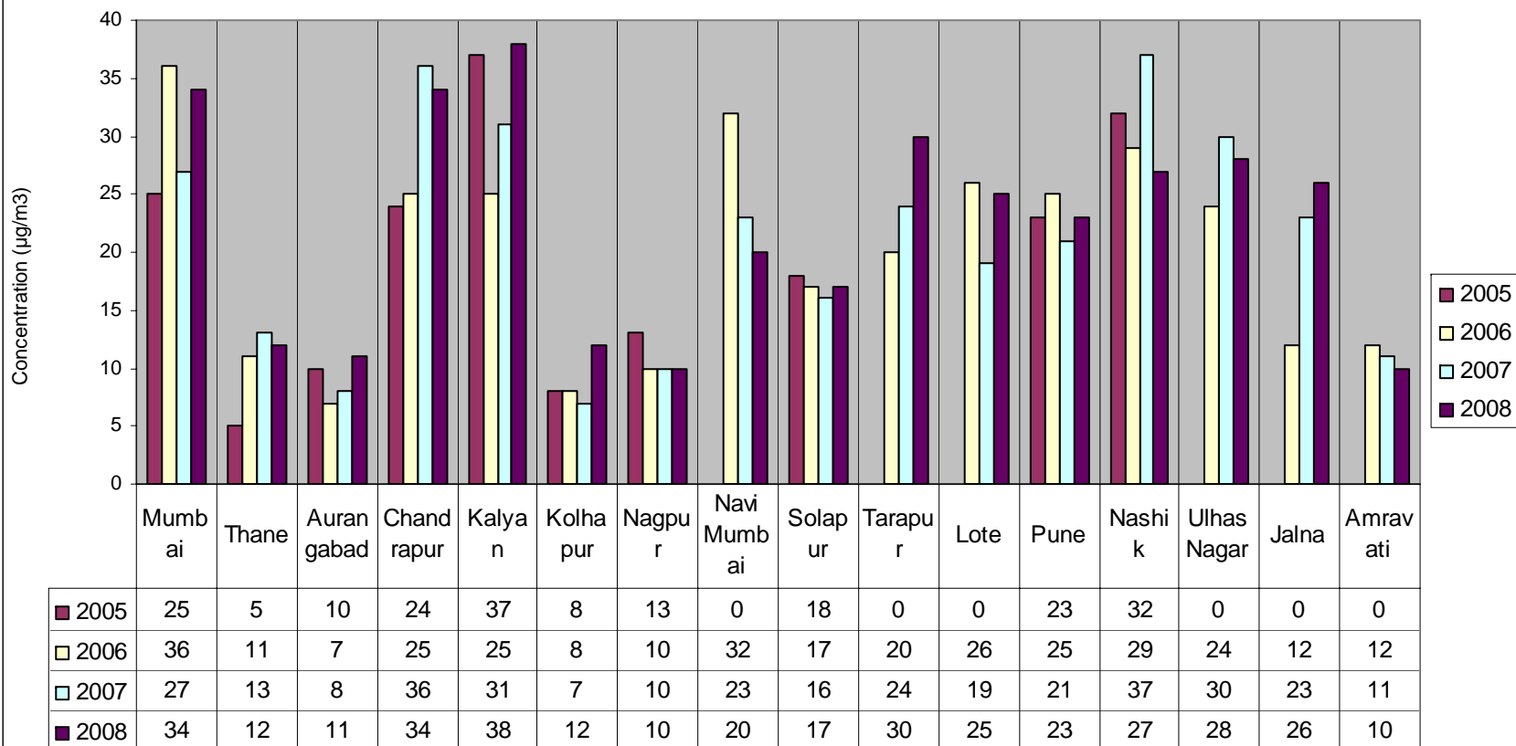
Trend in annual average concentration of SO 2 2005-2008
